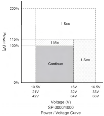
Figure 2. SP-3000/4000 Output power vs. input voltage
