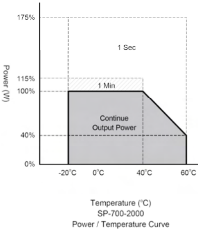
Figure 3. SP-700~2000 Output power vs. temperature
