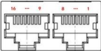
CAN & RS485
