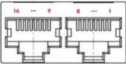
CAN & RS485
